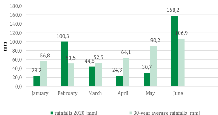
monthly rainfalls
