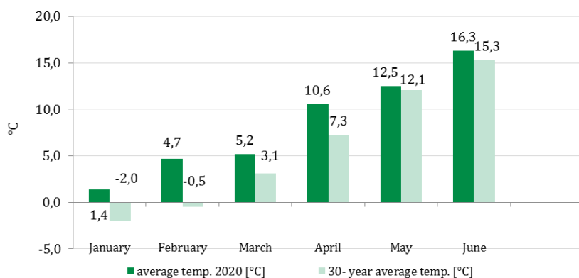
monthly temperature
