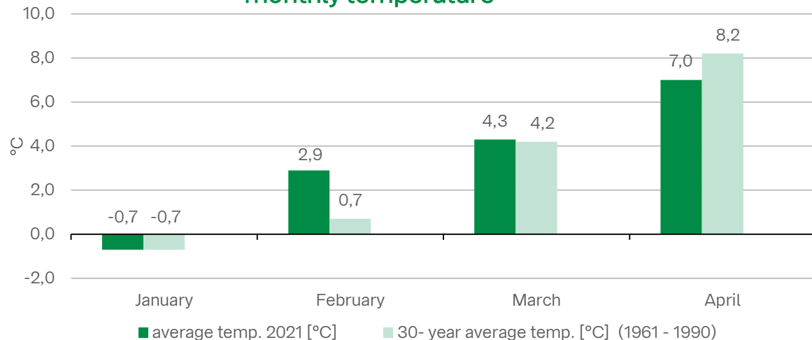
monthly temperature
