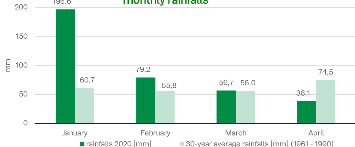
monthly rainfalls
