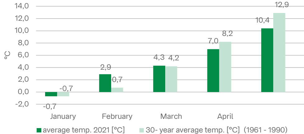
monthly temperature
