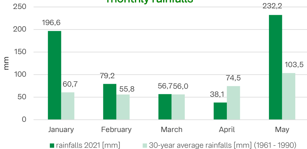
monthly rainfalls
