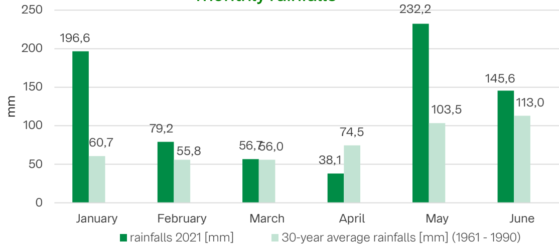
monthly rainfalls
