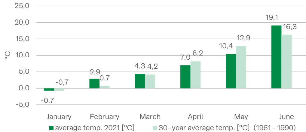
monthly temperature
