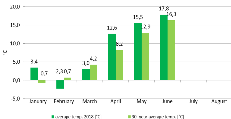
monthly temperature
