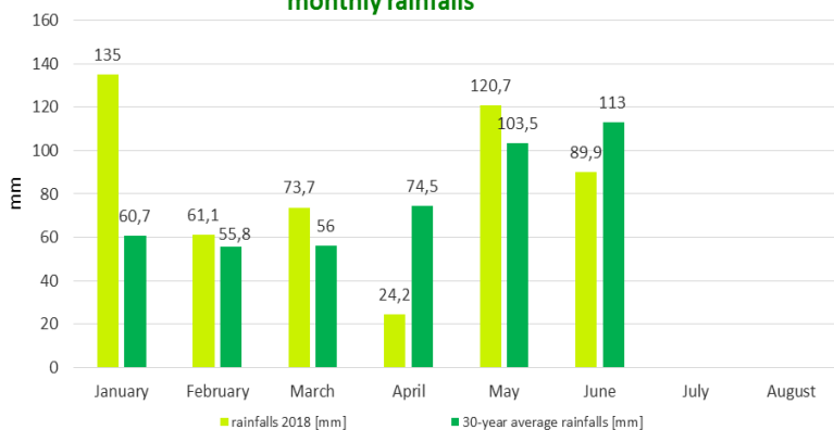
monthly rainfalls
