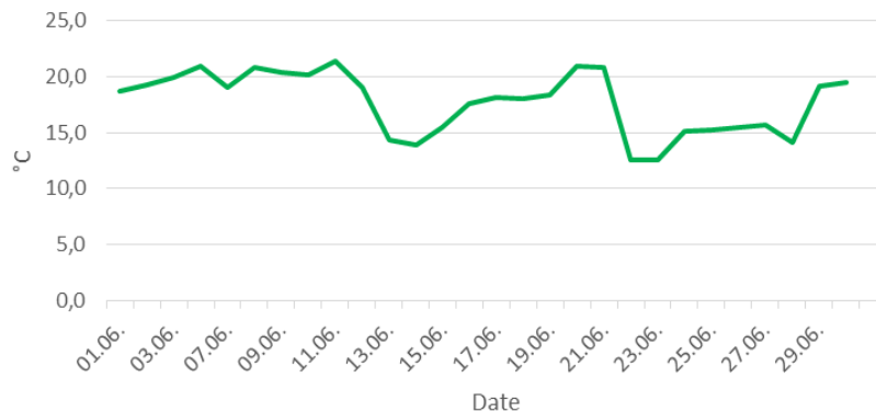
monthly temperature
