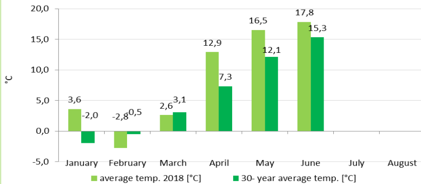
monthly temperature
