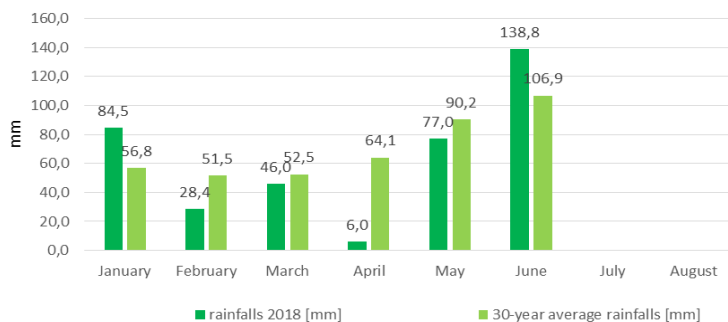
monthly rainfalls
