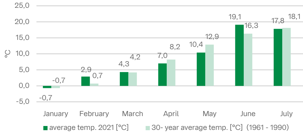
monthly temperature
