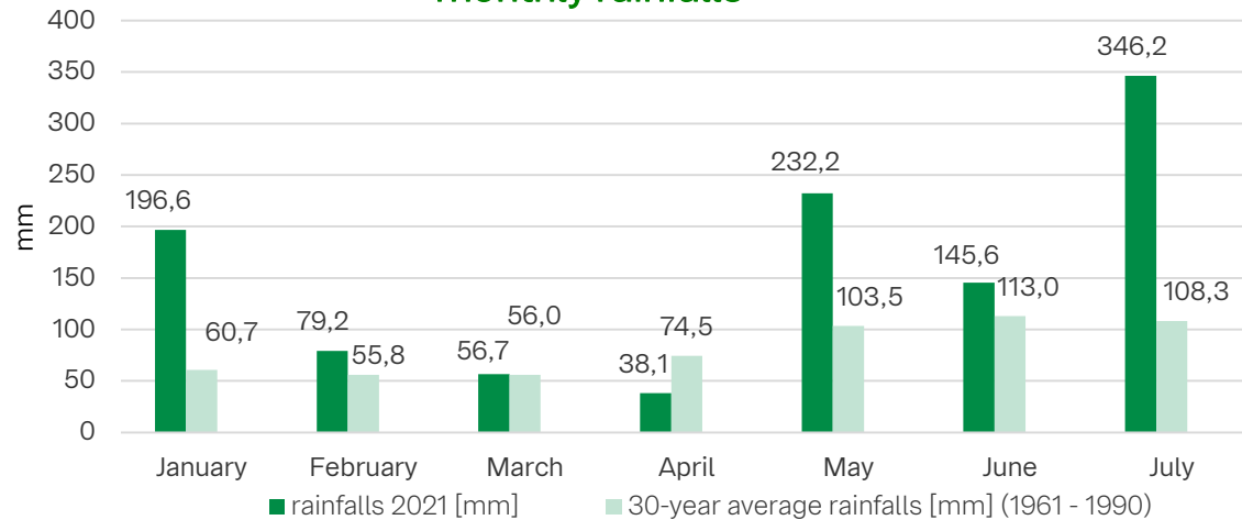
monthly rainfalls
