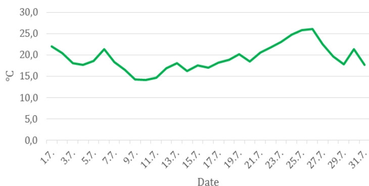
daily temperatures in July 2019
