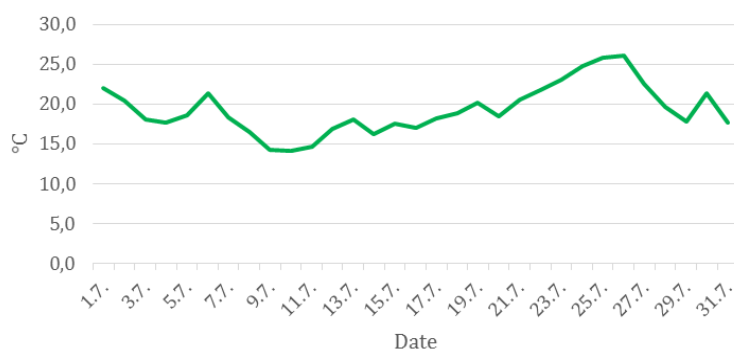
daily temperatures in July 2019
